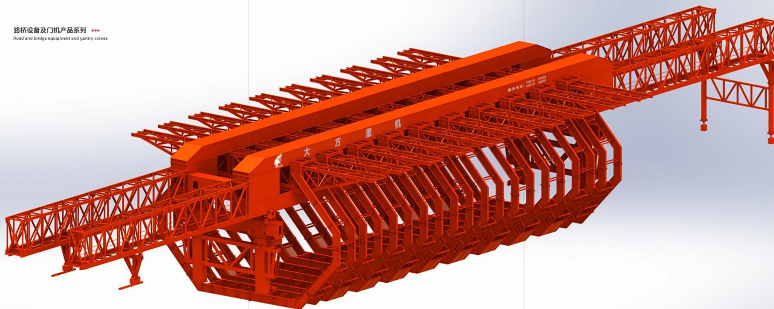
移动桥式起重机 movable formwork
